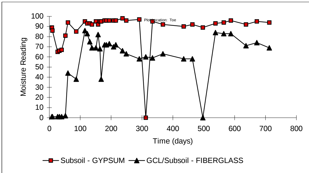
Figure D.9: MOISTURE READINGS VS. TIME FOR PLOT I (Bentofix NW - 2:1 Slope)
