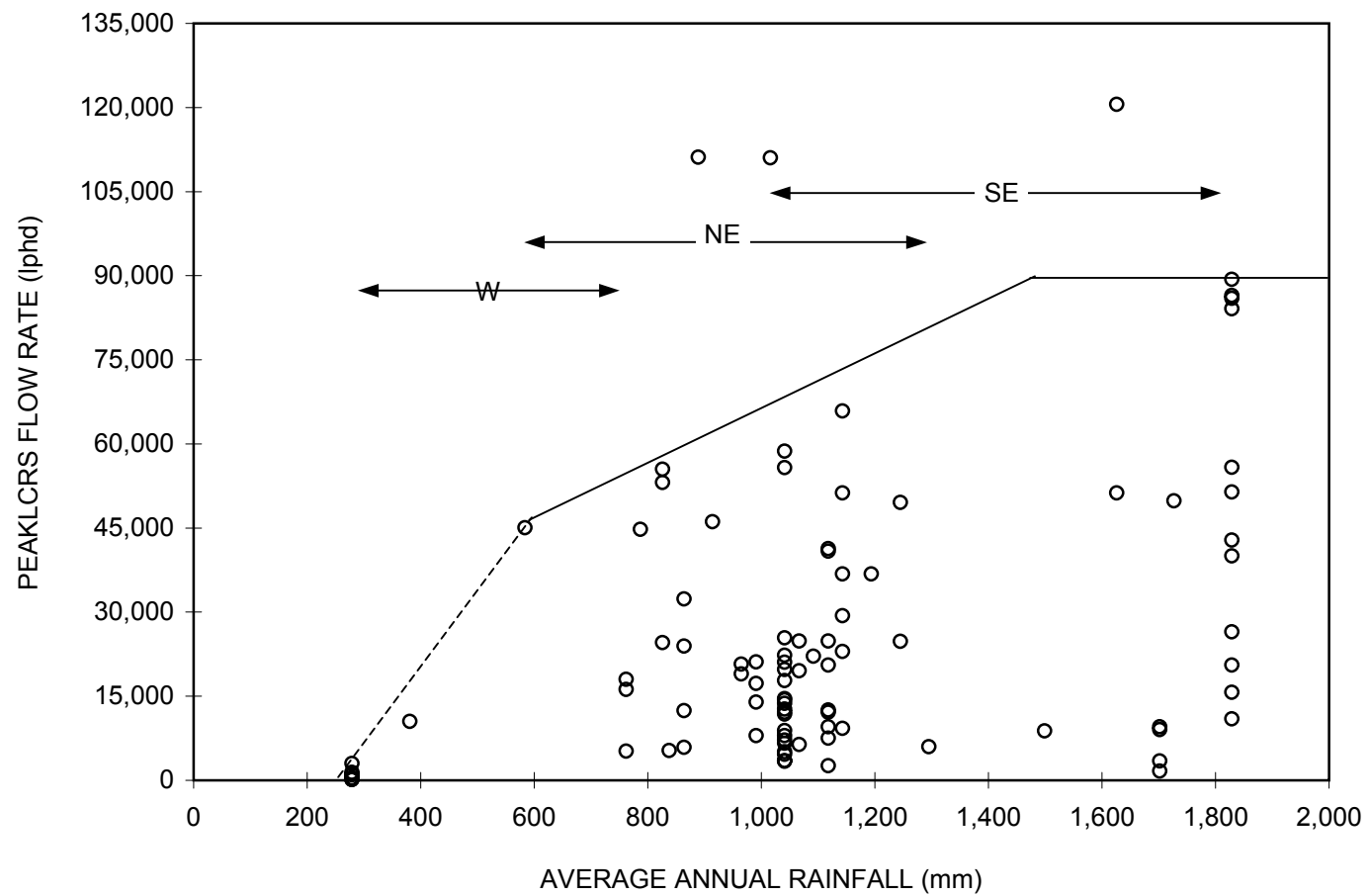
Figure E-5.2. Peak LCRS Flow Rate Versus Average Annual Rainfall During the Initial Period of Operation.
