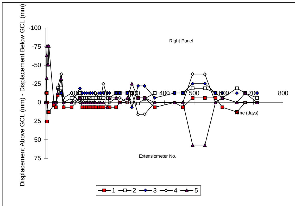
Figure C.9: RELATIVE DISPLACEMENT VS. TIME FOR PLOT I (Bentofix NW - 2:1 Slope)
