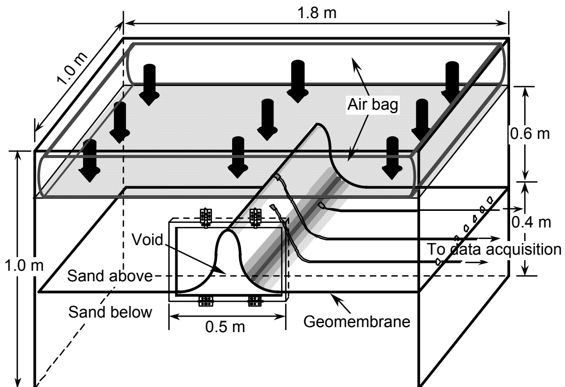
Figure 2-5. Photograph and schematic illustration of the large-scale experimental test box used in wave study.
