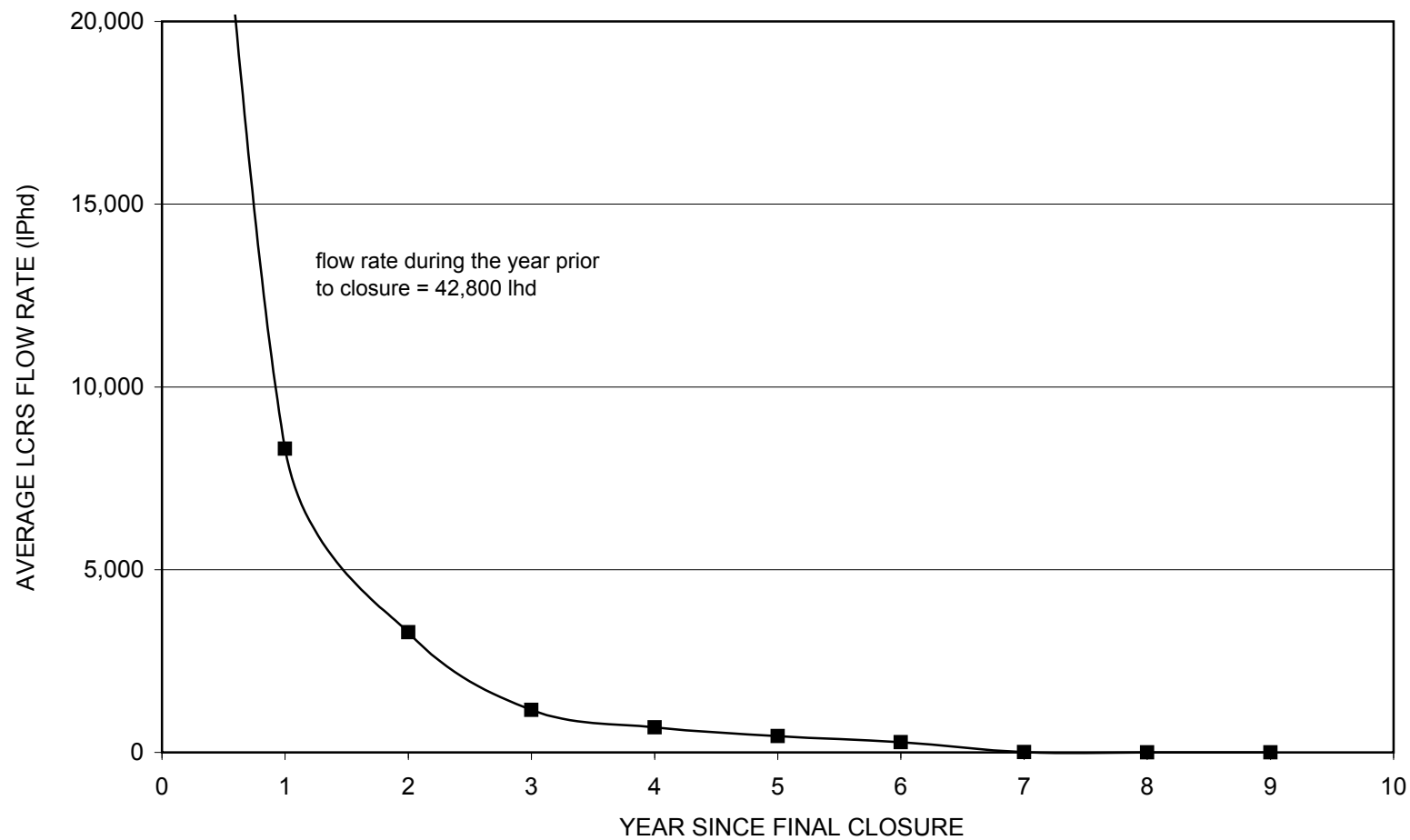
Figure E-5.5. Average LCRS Flow Rates (lhd) After Closure of Cell AD5, a HW Cell Located in the SE.
