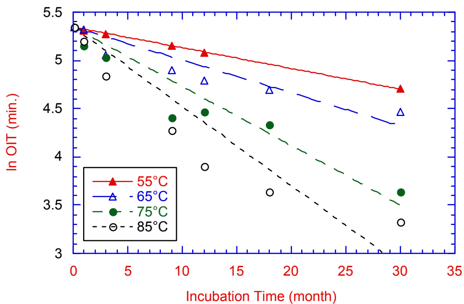
Figure B-14. Ln(OIT) versus incubation time plot for incubation series I using HP-OIT test.
