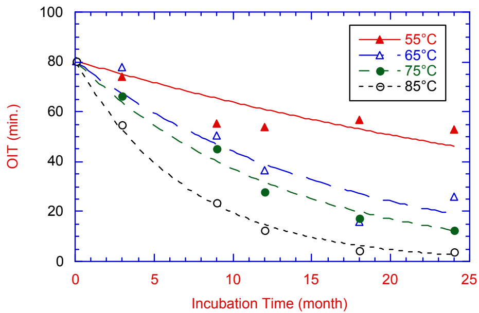
Figure B-16. Standard OIT versus incubation time plot for incubation Series III.
