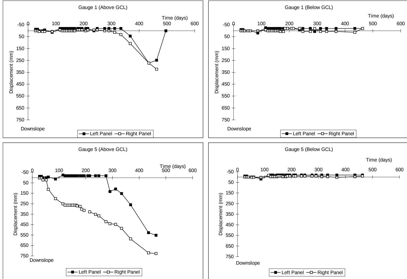
Figure A.6: POST-CONSTRUCTION DISPLACEMENT VS. TIME FOR PLOT F (Gundseal - Bentonite Side Up - 2:1 Slope)
