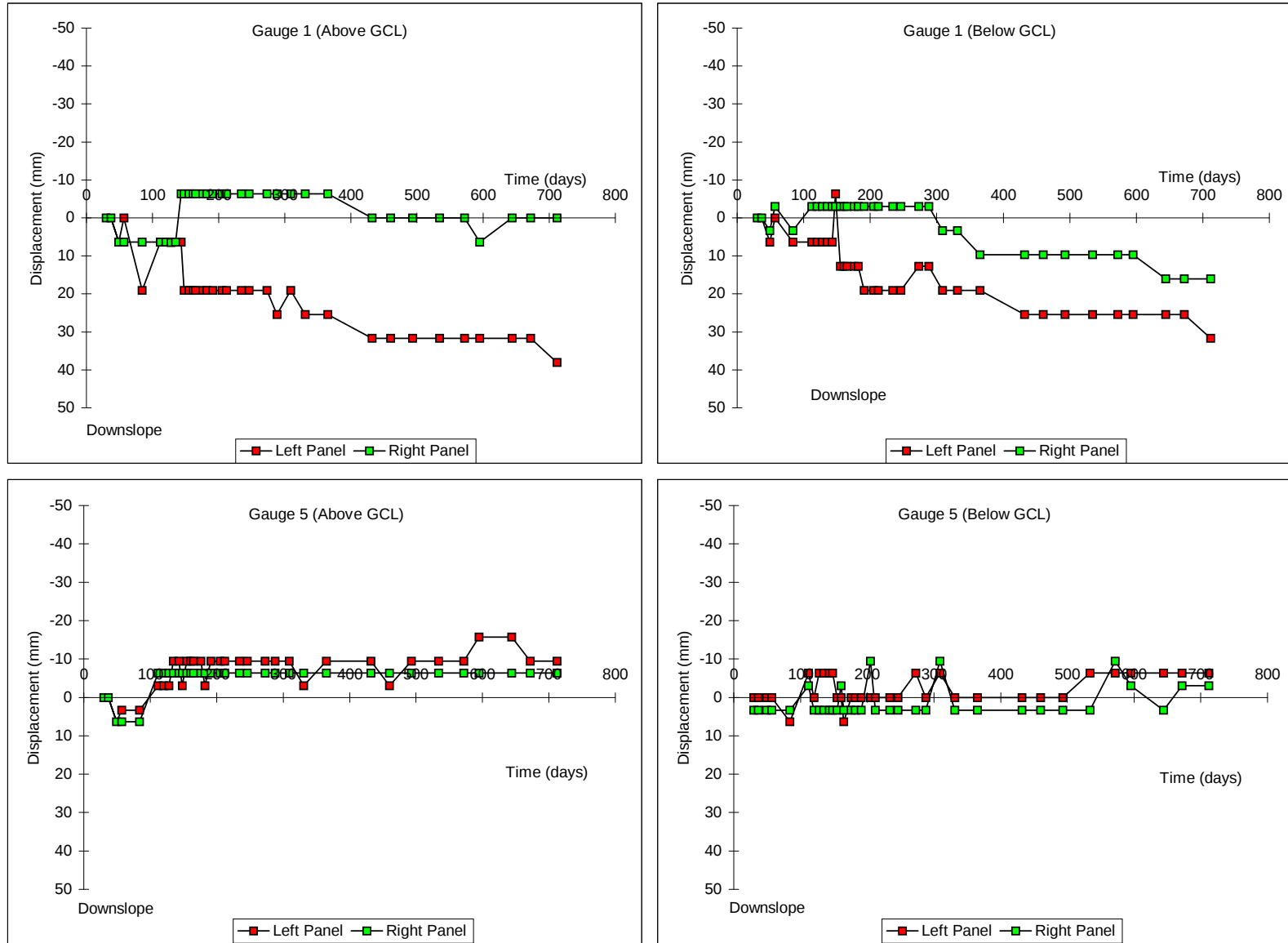
Figure A.4: POST-CONSTRUCTION DISPLACEMENT VS. TIME FOR PLOT D (Bentofix II (NW up) - 3:1 Slope)
