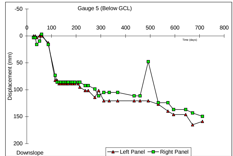
Figure A.9: POST-CONSTRUCTION DISPLACEMENT VS. TIME FOR PLOT I (Bentofix I - 2:1 Slope)
