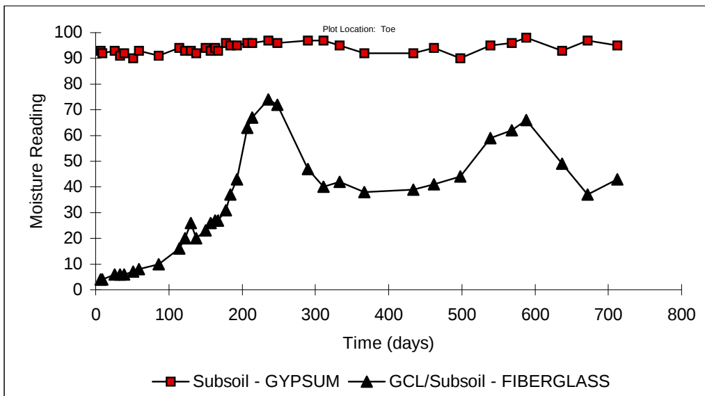
Figure D.12: MOISTURE READINGS VS. TIME FOR PLOT L (Bentofix NW - Granular Drainage - 2:1 Slope)
