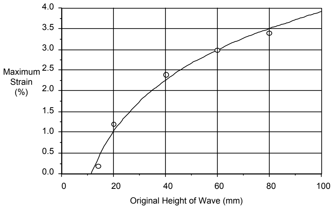
Figure A-27. Effect of original height of wave on the maximum strain measured at the end of experiments of HDPE GM waves.
