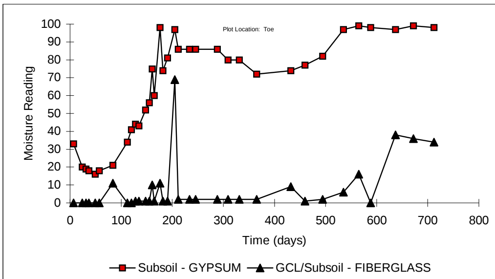
Figure D.4: MOISTURE READINGS VS. TIME FOR PLOT D (Bentofix NS - 3:1 Slope)
