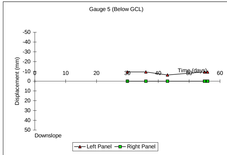
Figure A.7: POST-CONSTRUCTION DISPLACEMENT VS. TIME FOR PLOT G (Bentomat - 2:1 Slope)
