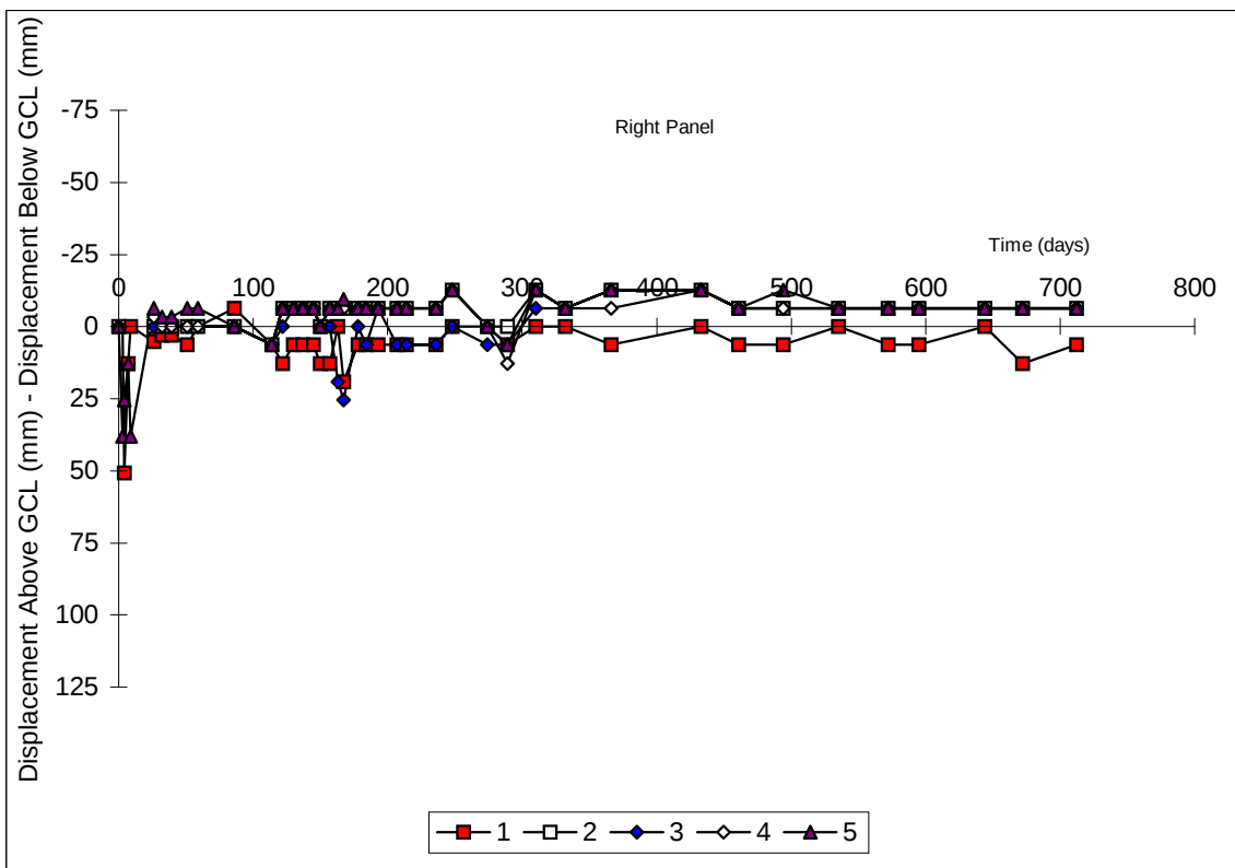
Figure C.12: RELATIVE DISPLACEMENT VS. TIME FOR PLOT L (Bentofix NW - Granular Drainage - 2:1 Slope)
