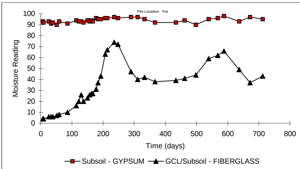
Figure D.12: MOISTURE READINGS VS. TIME FOR PLOT L (Bentofix NW - Granular Drainage - 2:1 Slope)
