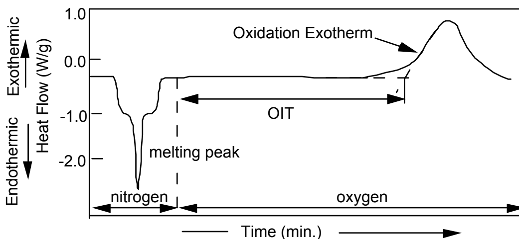
Figure B-9. Thermal curve of a standard OIT test.
