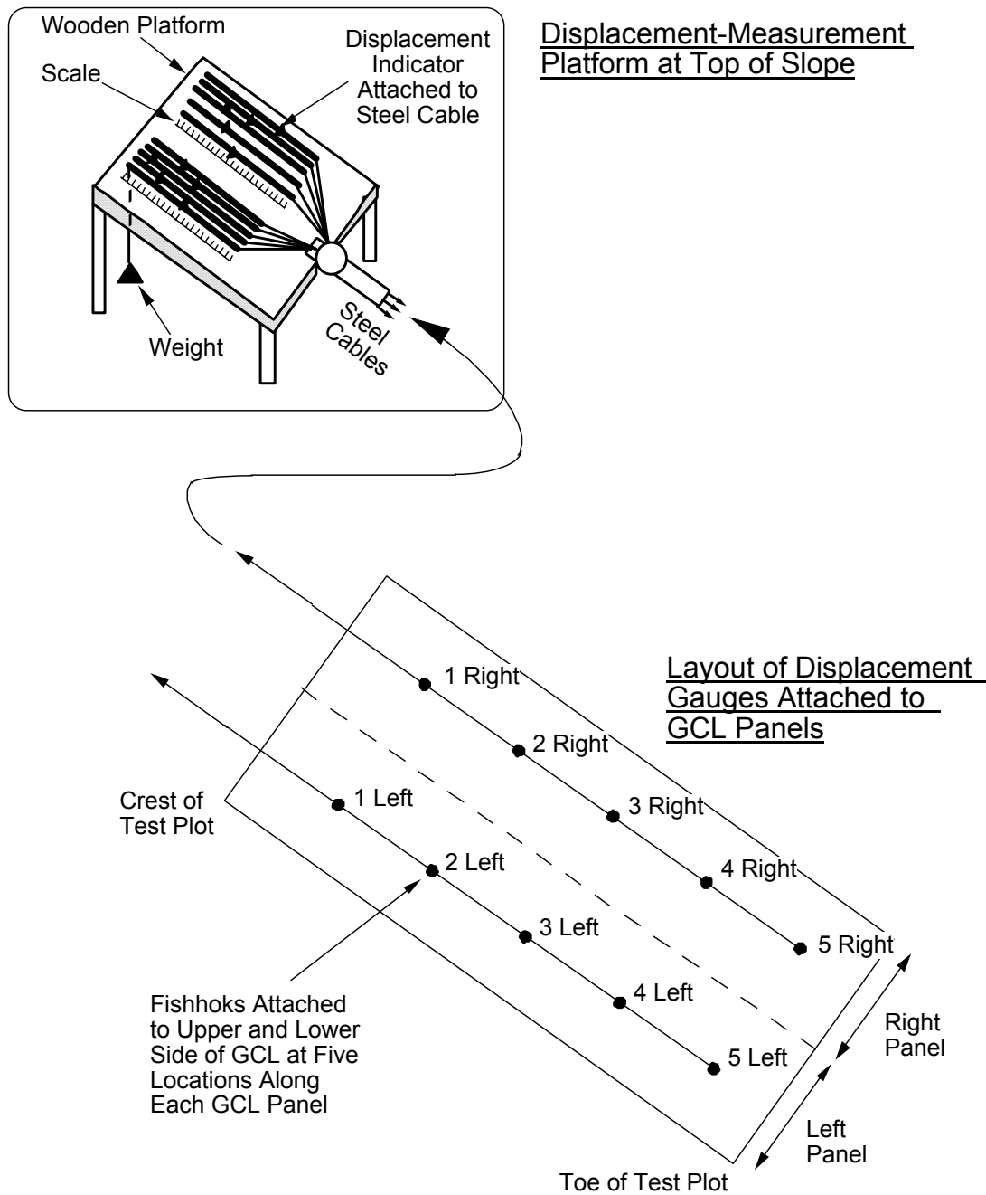
Figure 3-19. Displacement monitoring system.
