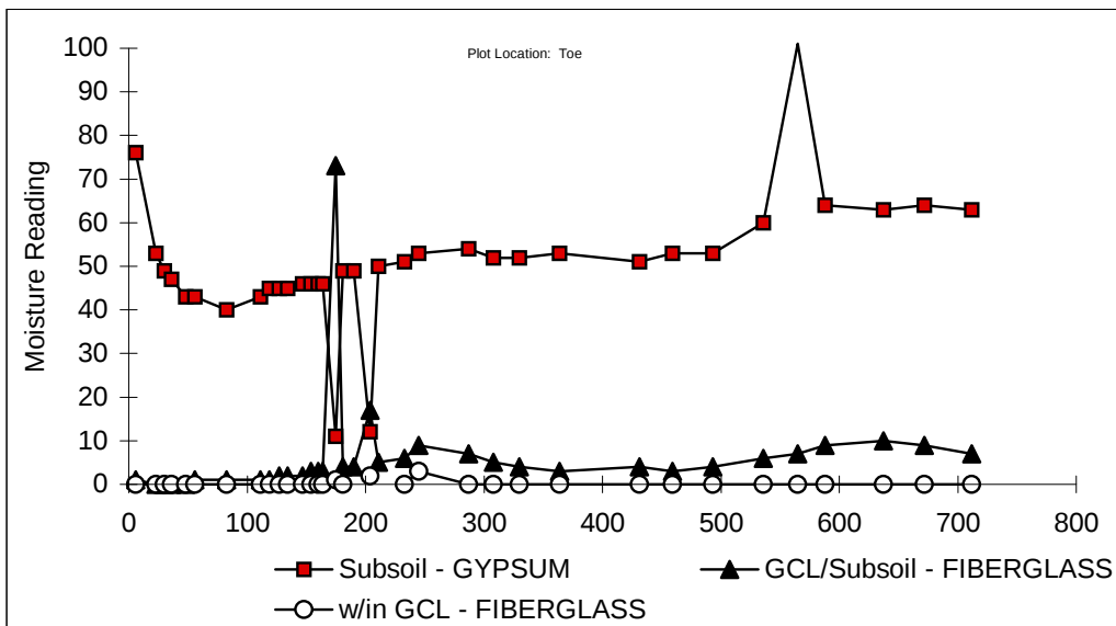
Figure D1: MOISTURE READINGS VS. TIME FOR PLOT A (Gundseal - Bentonite up - 3:1 Slope)
