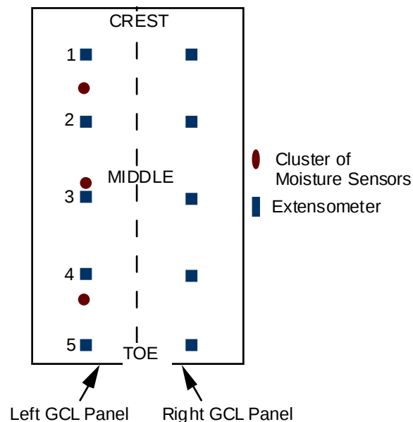
Figure D-12. Locations of moisture sensors and extensiometers.
